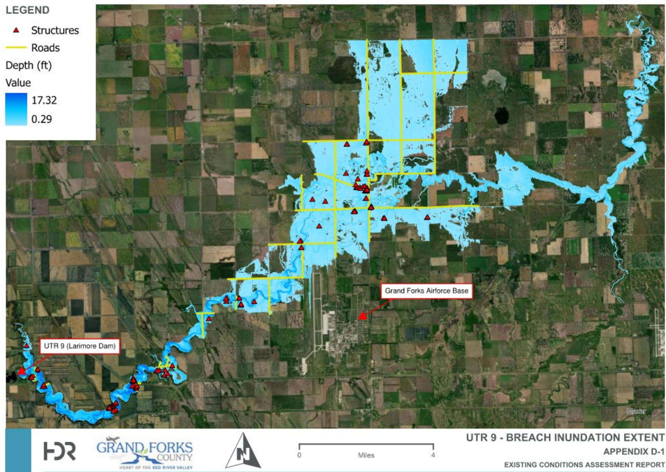
Appendix C-6: Breach Inundation, Hazard Class Analysis - Overall
