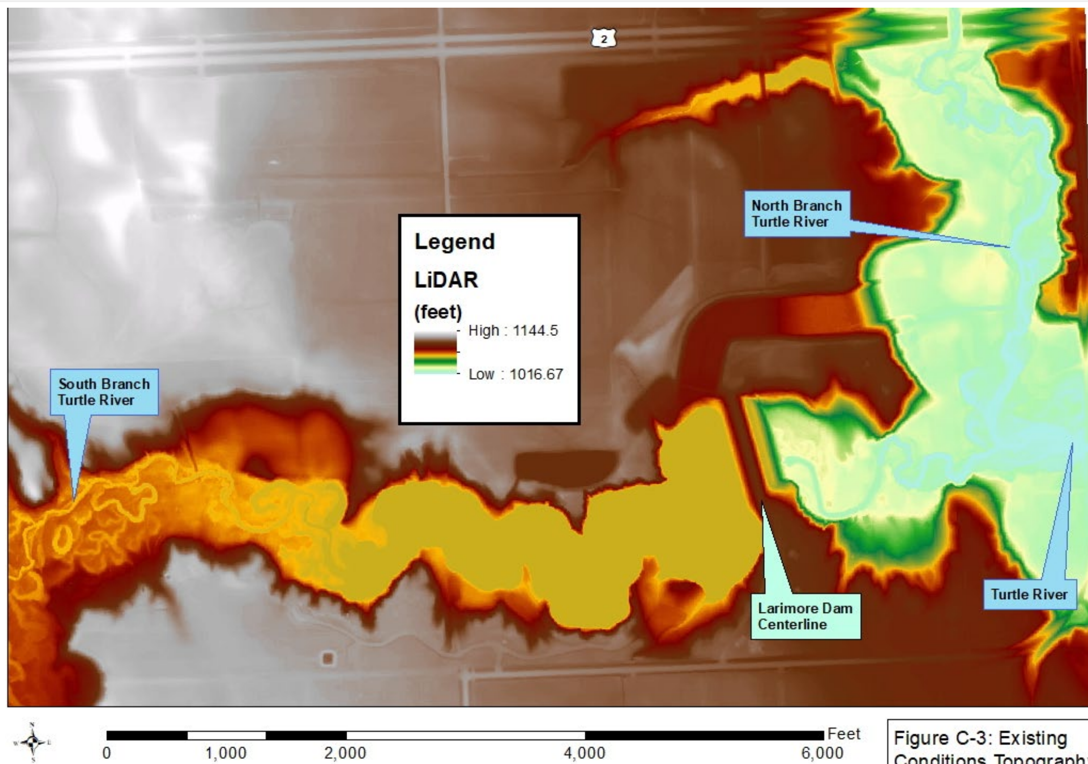
Appendix C-3: Existing Topography
