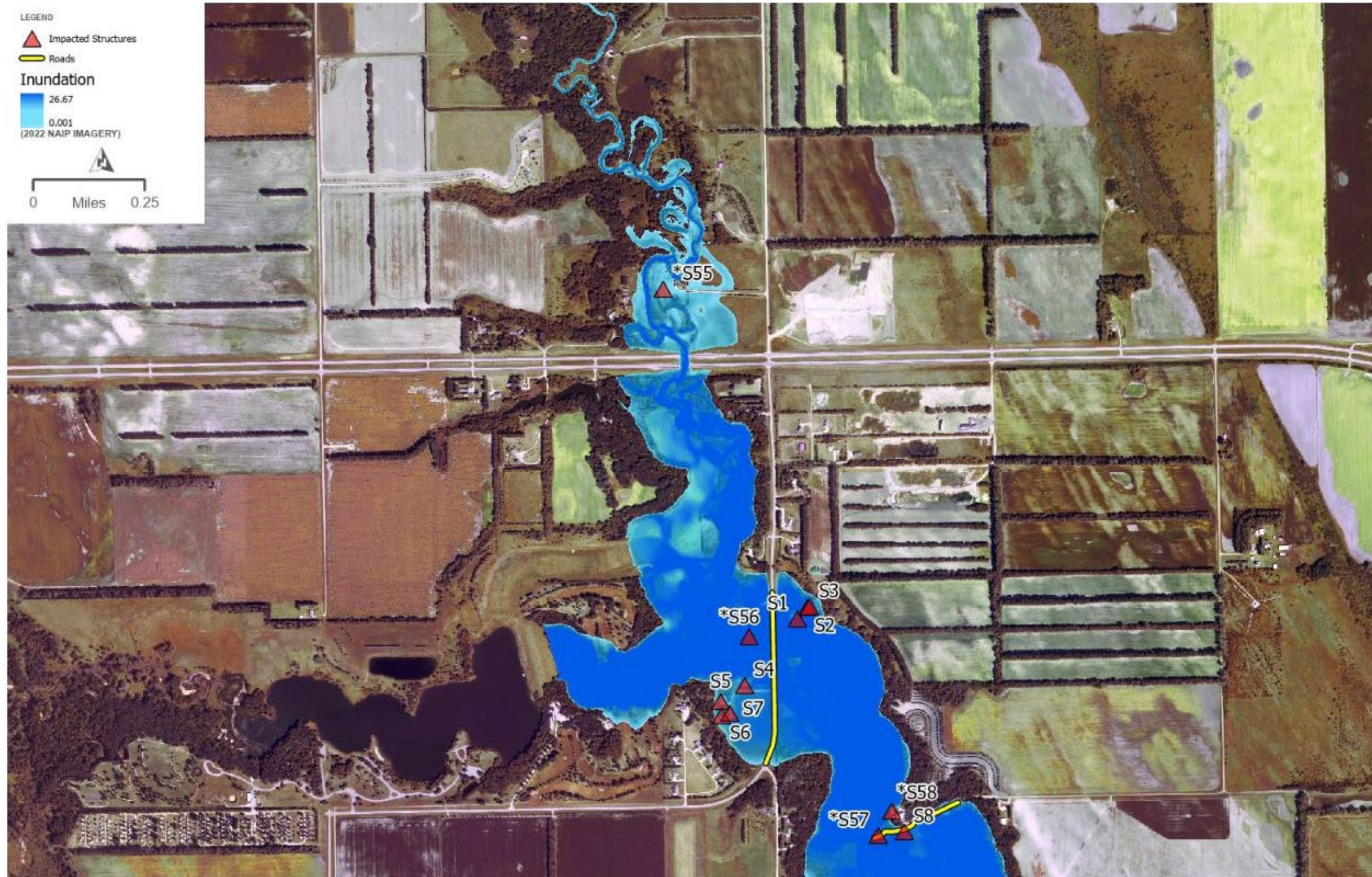
Appendix C-7: Breach Inundation, Hazard Class Analysis - 1
