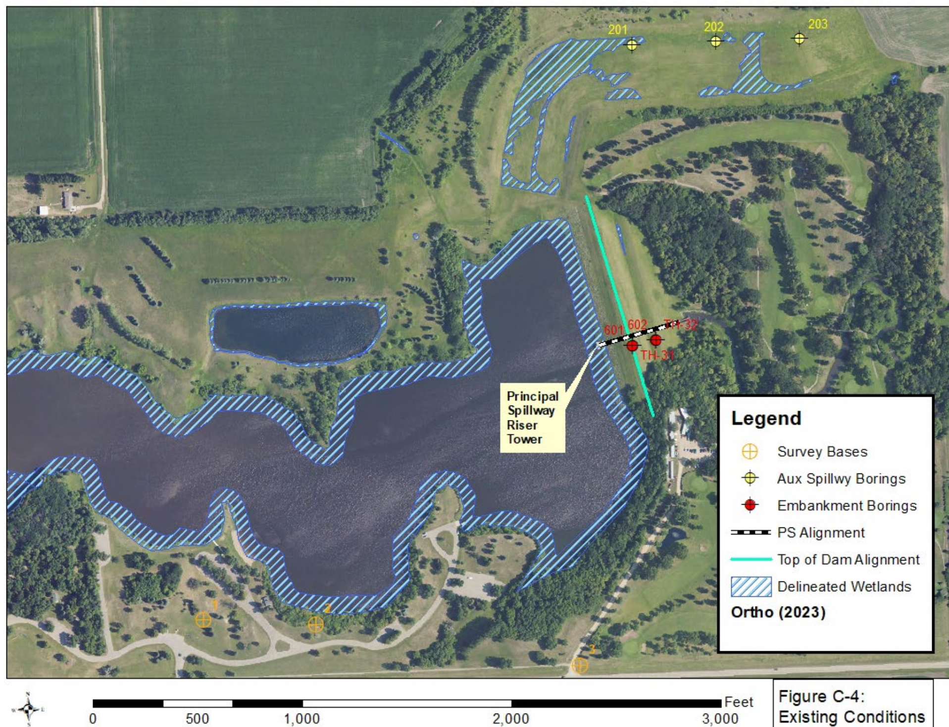
Appendix C-4: Existing Conditions Overall Site Plan
