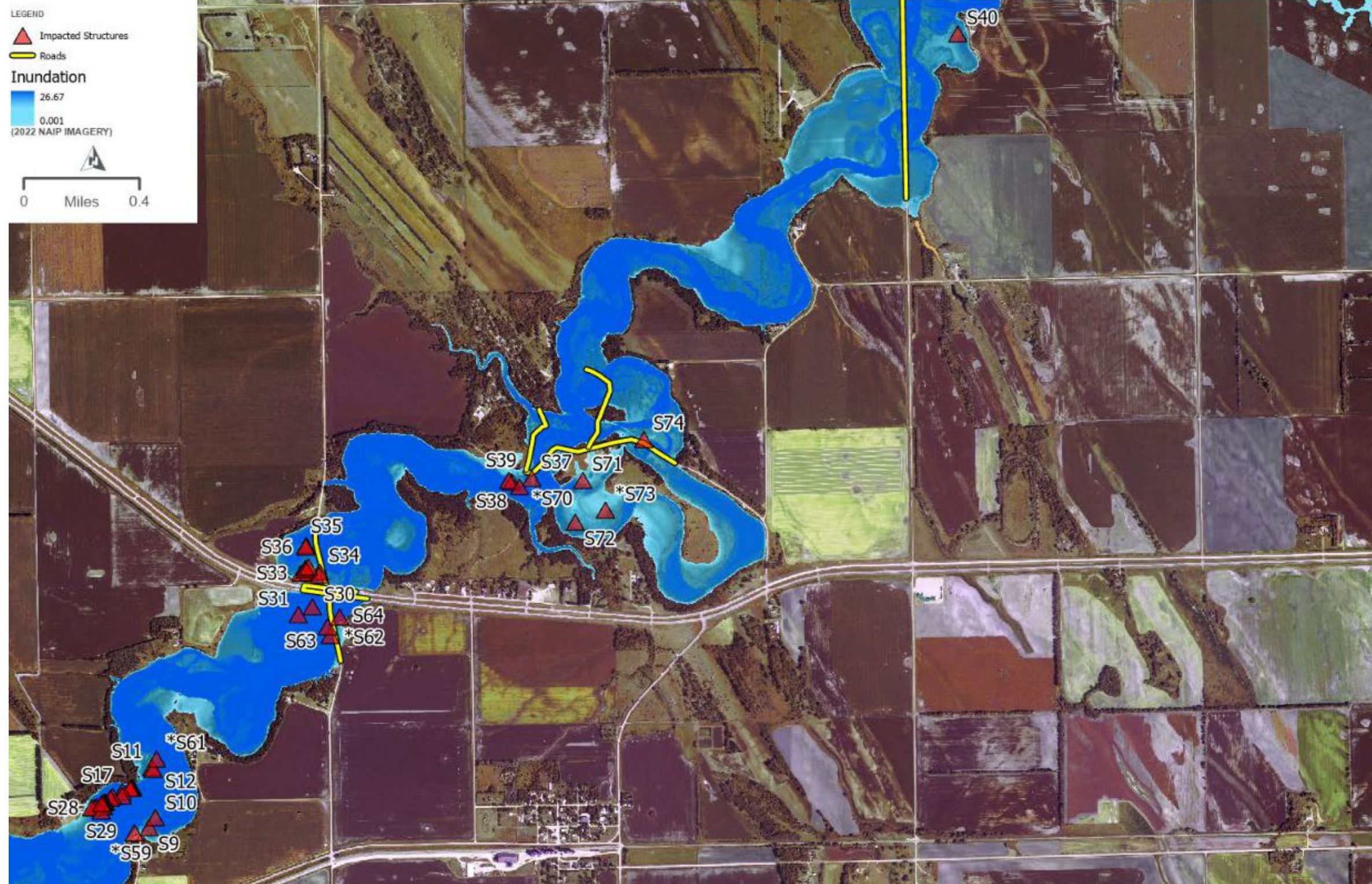
Appendix C-9: Breach Inundation, Hazard Class Analysis - 3
