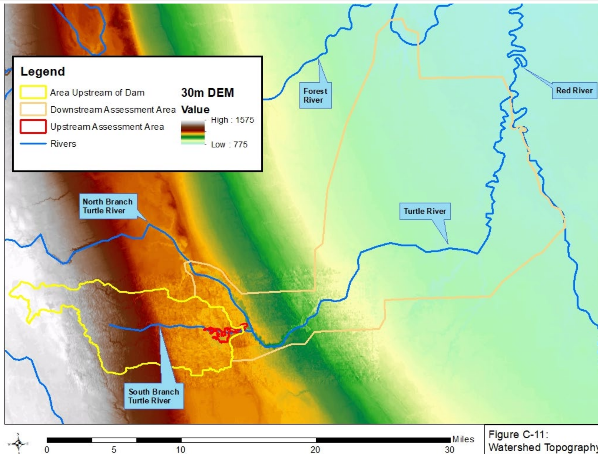
Appendix C-11: Watershed Topography
