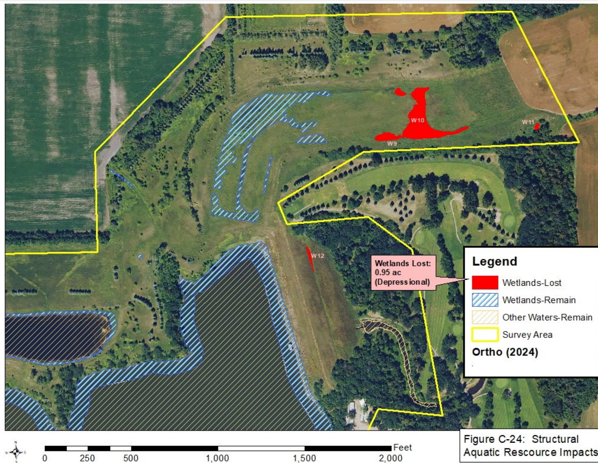
Appendix C-24: Preferred/Structural Alternative – Aquatic Resource Impacts Map (Permanent Impacts)
