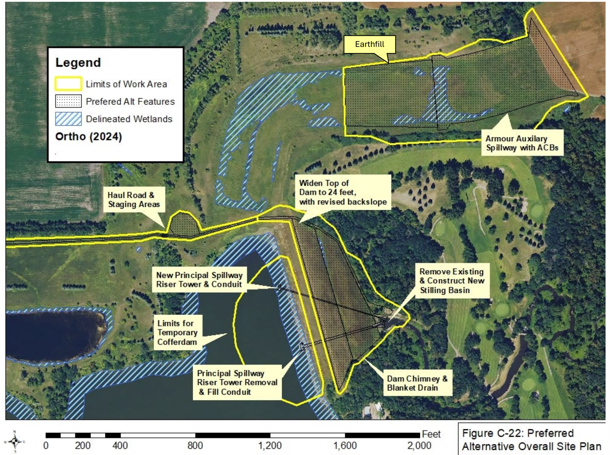
Appendix C-22: Preferred Alternative Overall Site Plan
