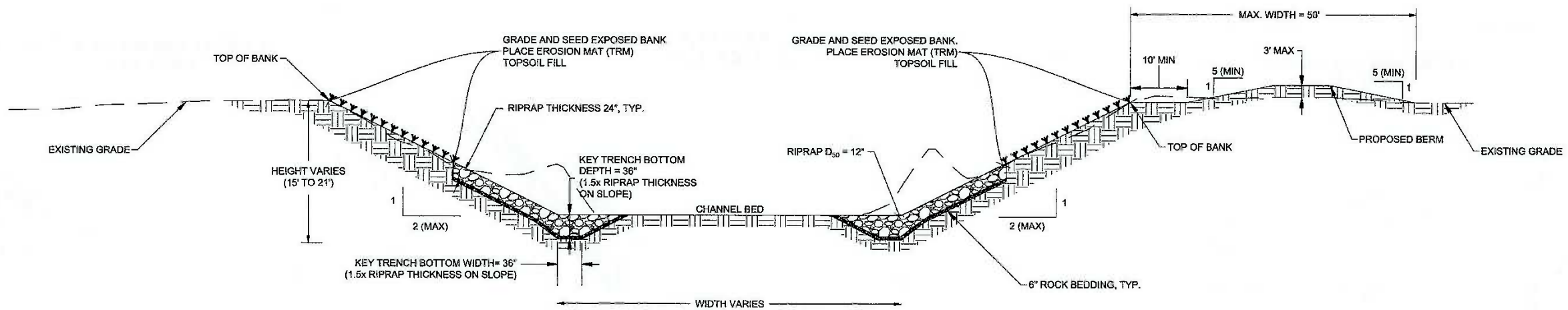
A2 BANK STABILIZATION DETAIL - HALF BANK OPTION NTS
