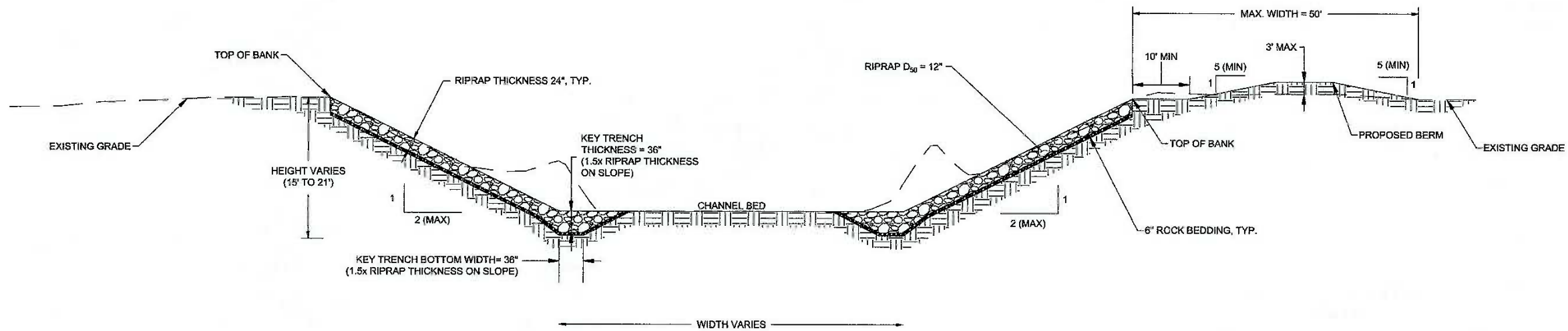
A1 BANK STABILIZATION DETAIL - FULL BANK OPTION NTS
