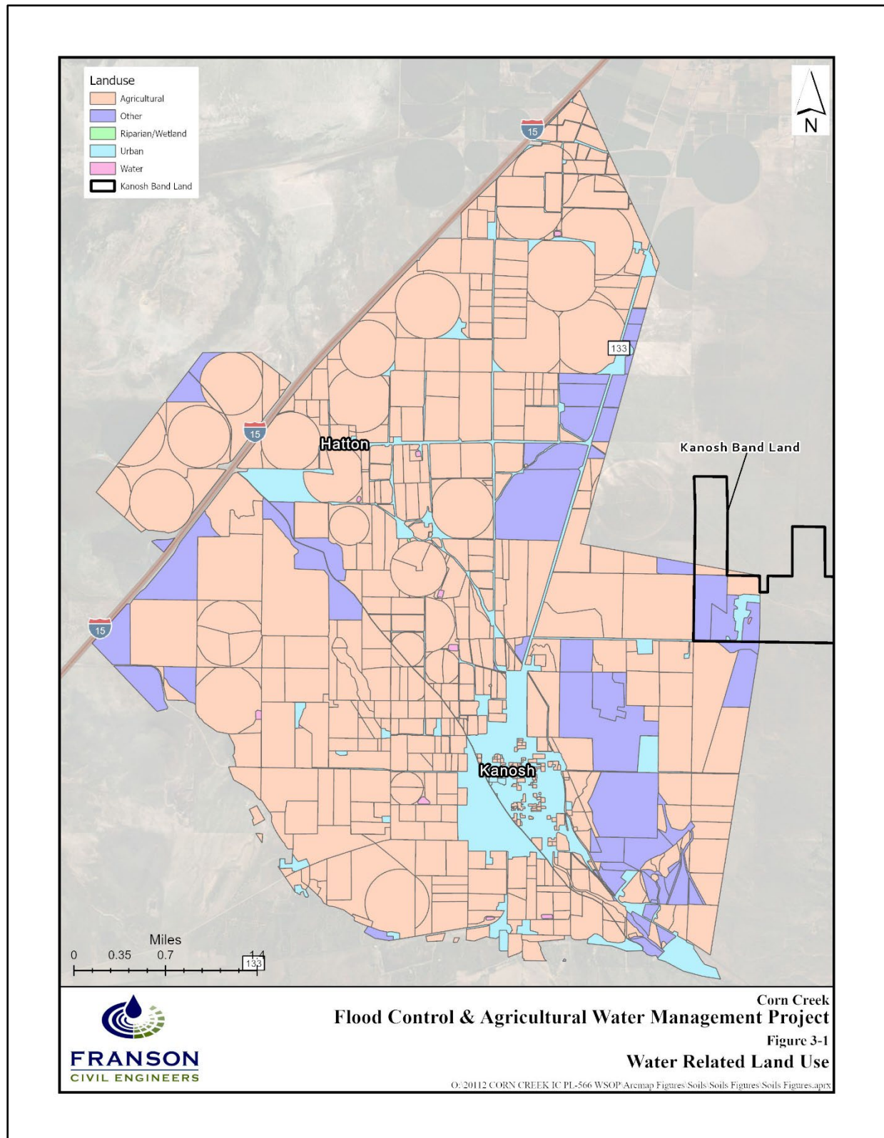
Figure 3-26: Water Related Land Use (UGRC 2023)
