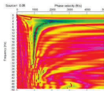
Figure 2 frequency vs velocity plot
