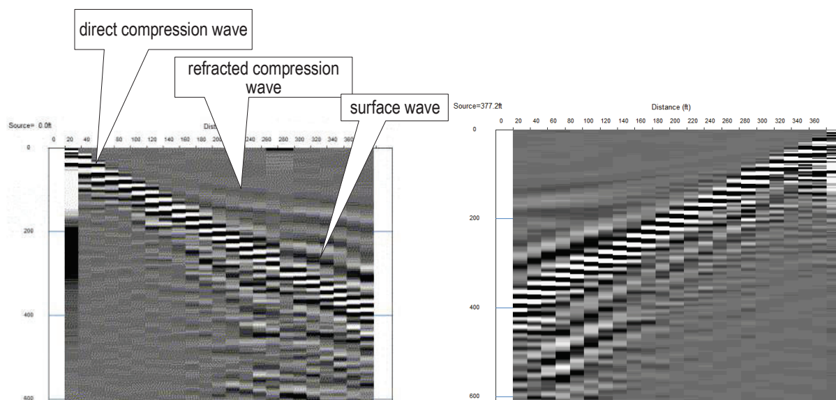
Figure 4. typical field records (truncated)
