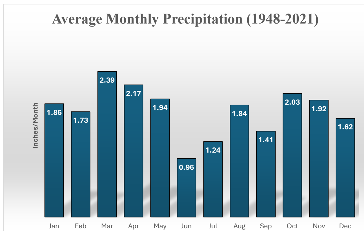
Figure 6: Corn Creek Watershed Average Precipitation (USGS StreamStats)
