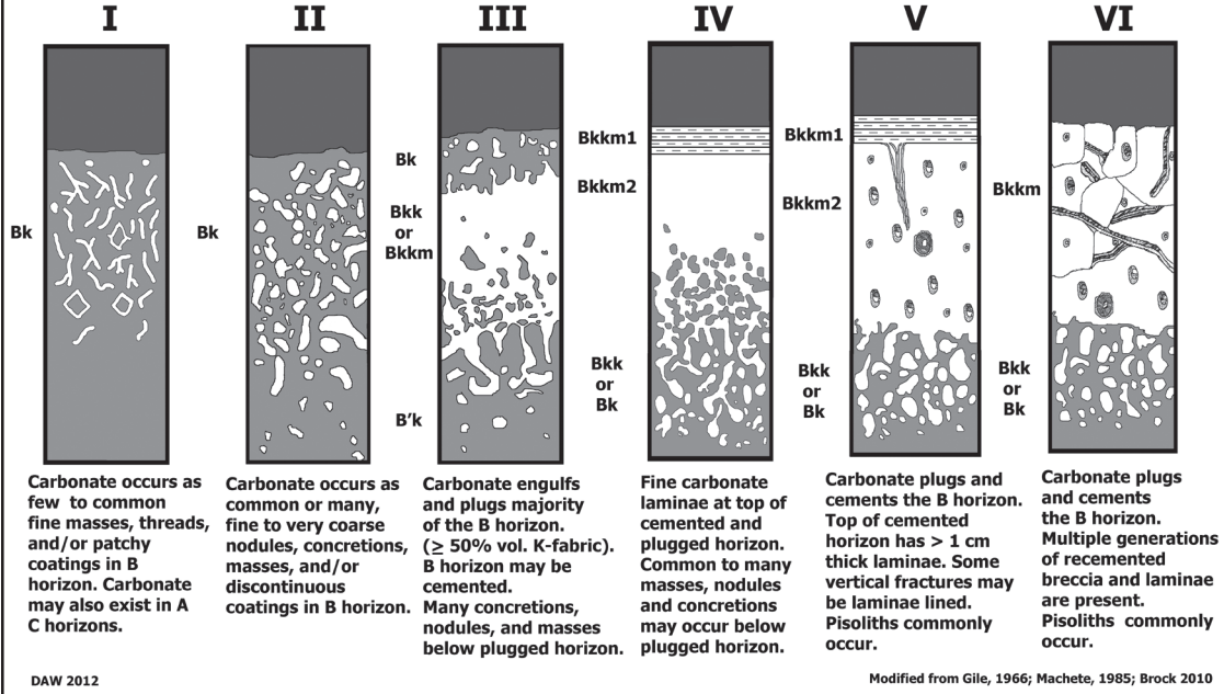
Figure A - Pedogenic Carbonate Development Stages - Fine Earth Matrix
