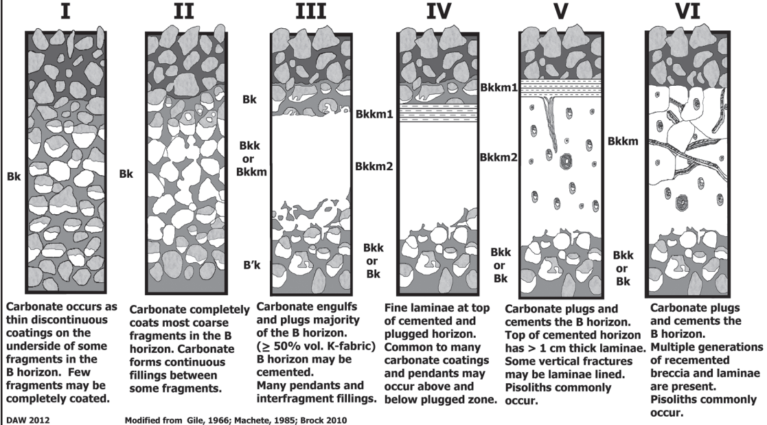
Figure B - Pedogenic Carbonate Development Stages - Coarse Fragment Matrix
