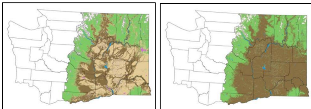
Left: Current extent of forest cover (green), shrubsteppe/grassland (brown), agriculture (tan), water (blue), and urban areas (magenta) in eastern Washington. Right: Historic extent shrubsteppe/grassland (brown) in eastern Washington.
