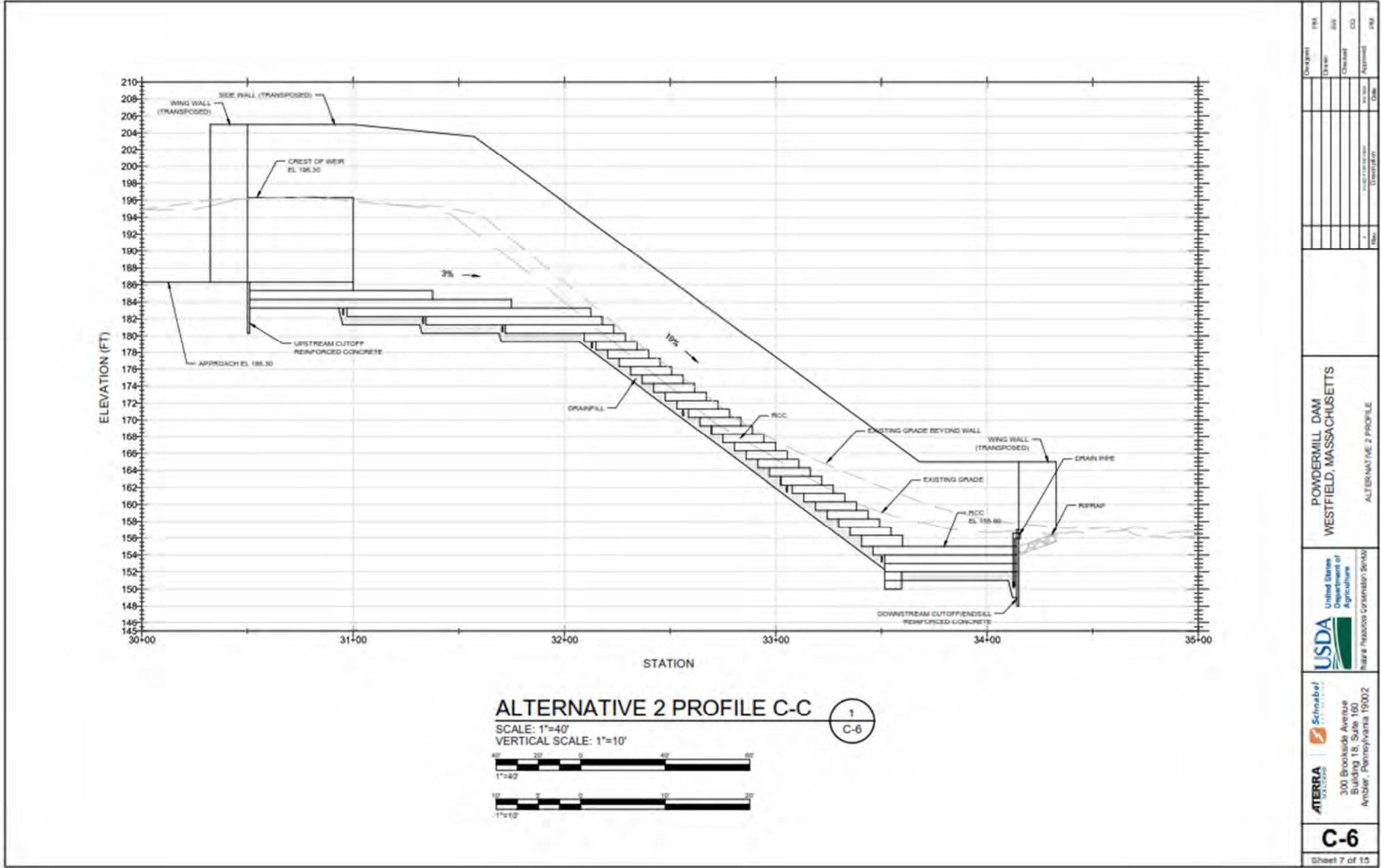
Figure C-24 - Profile View of Alternative 2
