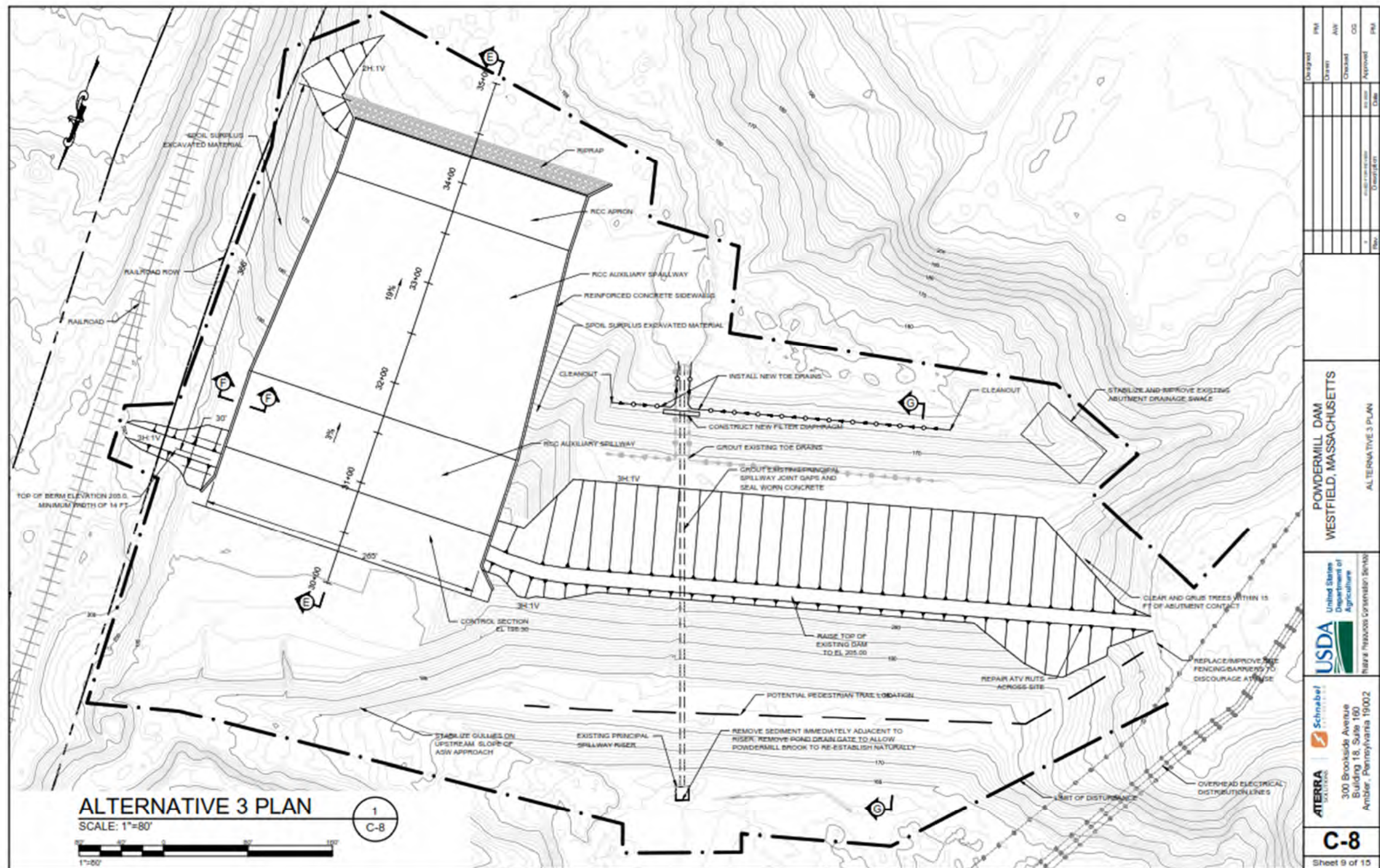
Figure C-26 - Plan View of Alternative 3
