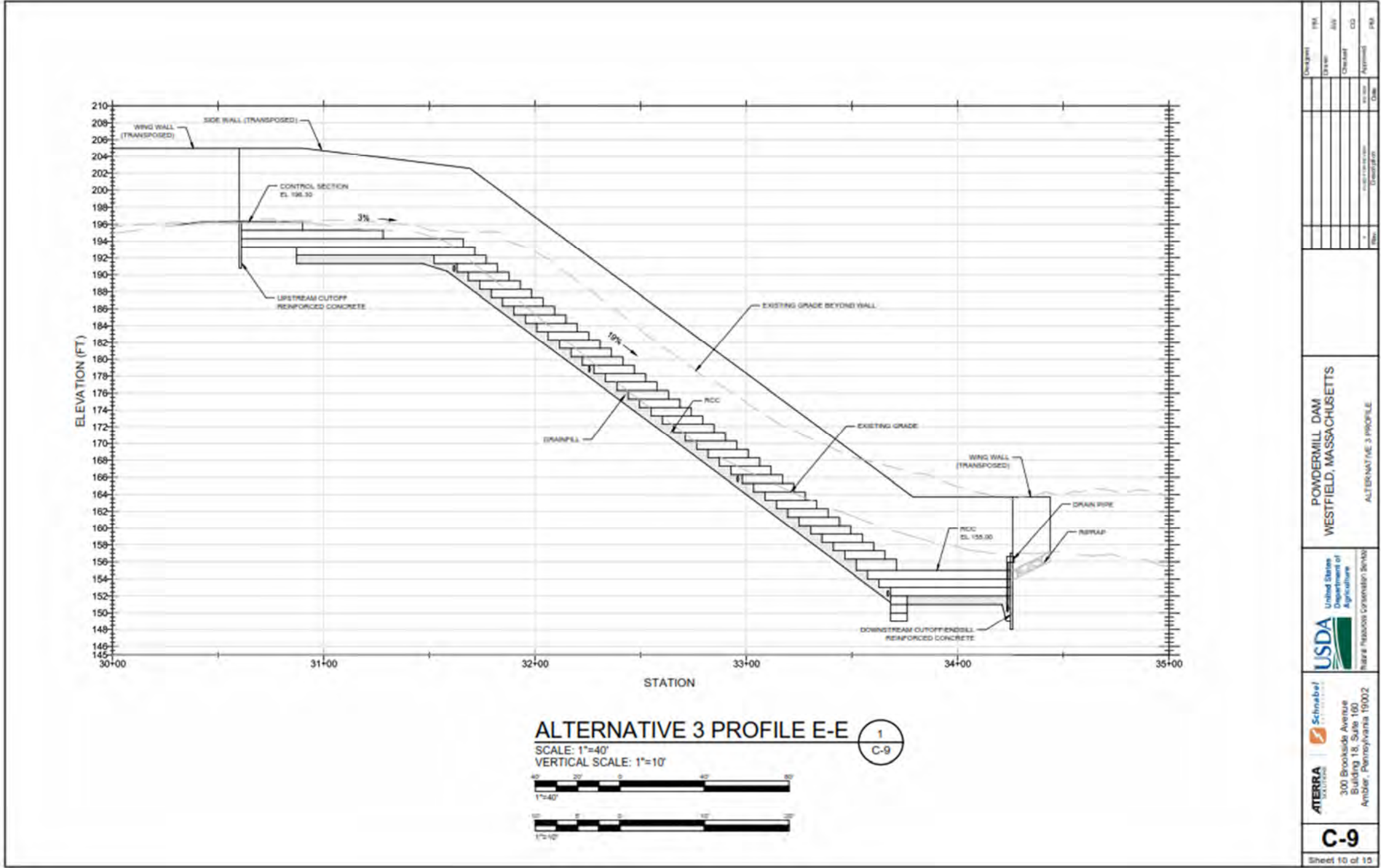
Figure C-27 - Profile View of Alternative 3
