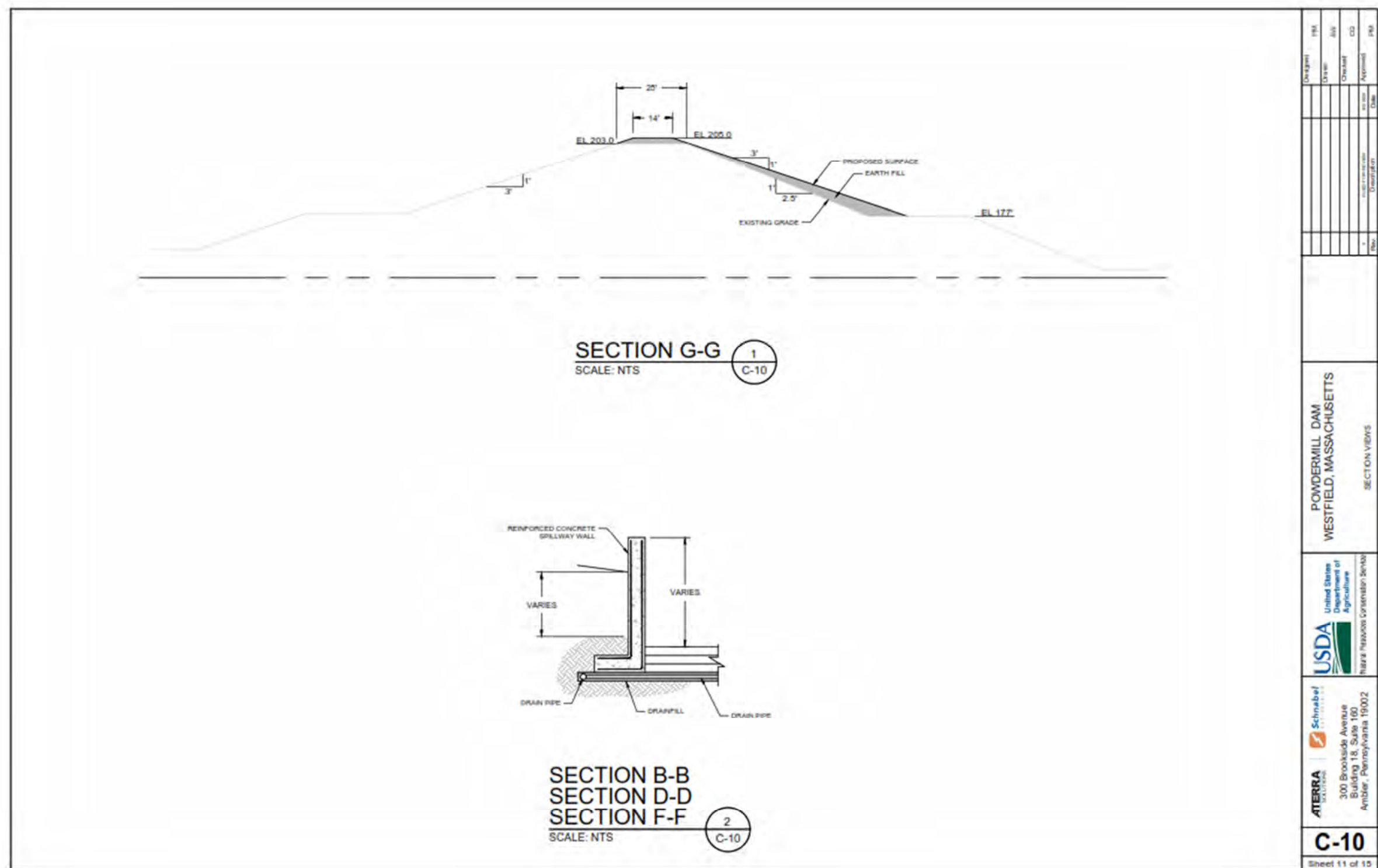
Figure C-28 – Details for Dam Raise and Training Wall
