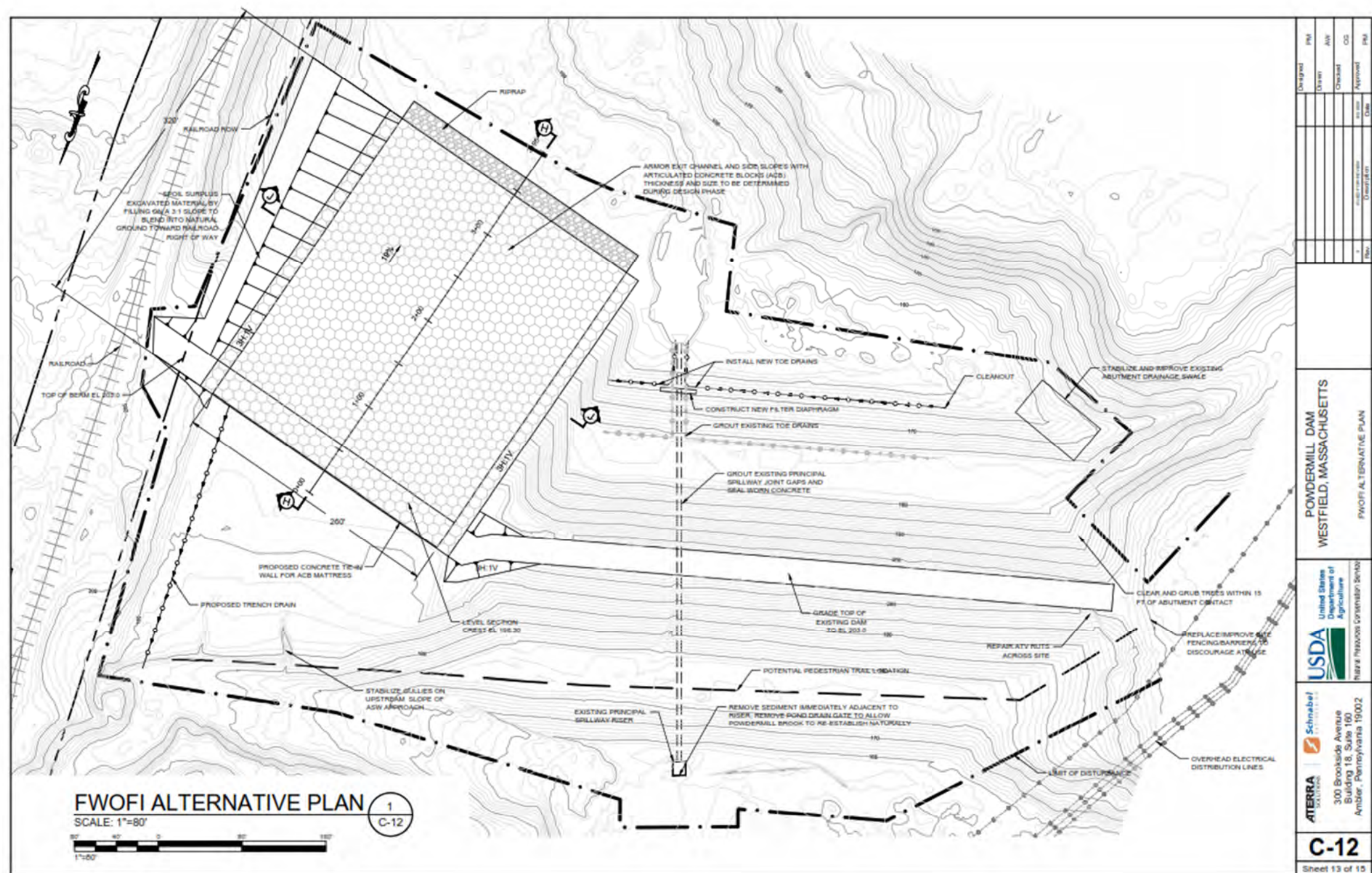
Figure C-30 – Plan View of FWOFI Alternative
