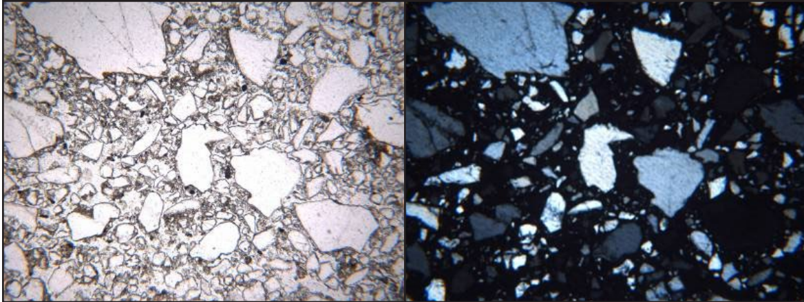
Figure 3E1b-8.—Enaulic c/f related distribution pattern. Material is from an E horizon of a Fuquay soil, which is a Kandiodult, in South Carolina (pedon 06N0830). Frame width is 2.5 mm. Light is plane-polarized on the left and cross-polarized on the right.
