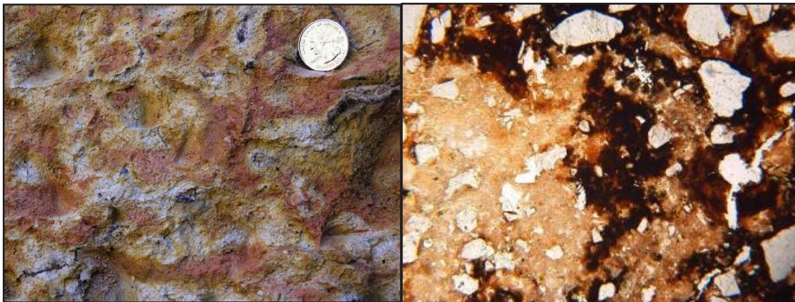
Figure 3E1b–18. —The mottled fabric on the pit face (left) and the thin section of soil fabric from the same horizon (right). These photos illustrate the movement of iron oxides in the soil as it undergoes seasonal saturation and reduction followed by reoxidation. Material is from a Btvx2 horizon of a Fuquay soil.
