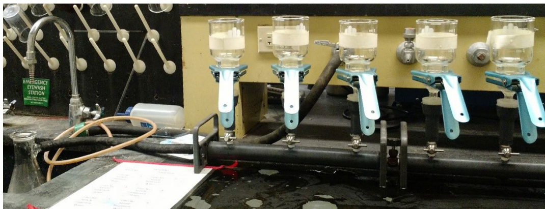
Figure 7A1-2.—Vacuum apparatus.
